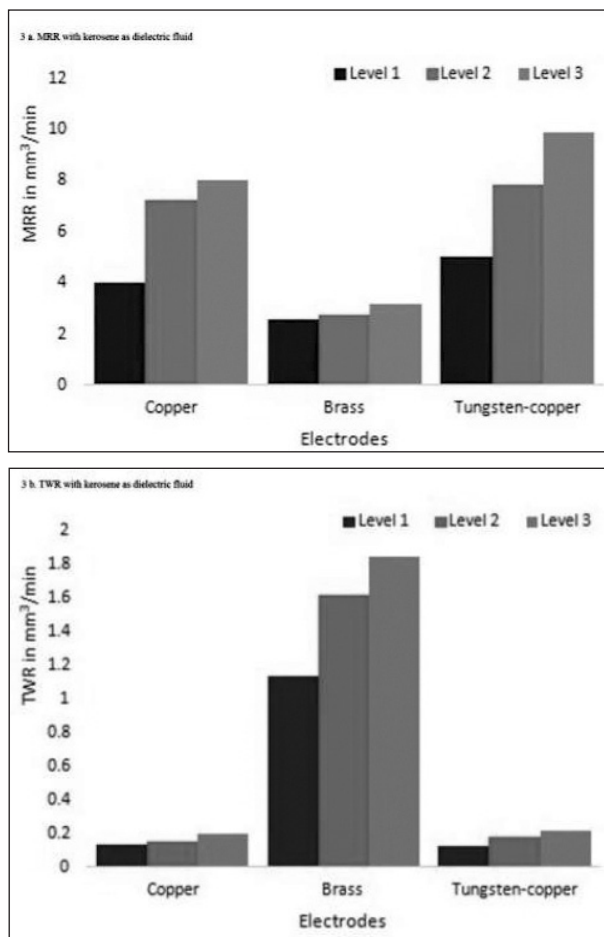
Fig. 3. a-c. MRR and TWR with kerosene as dielectric fluid.
