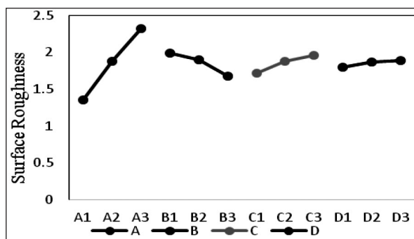
Fig. 1. Response graph for surface roughness.
