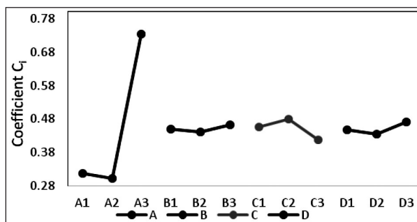
Fig. 4. Response graph for C i values.
