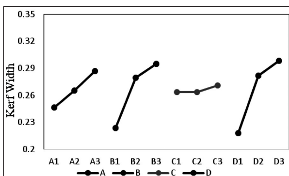
Fig. 3. Response graph for kerf width.
