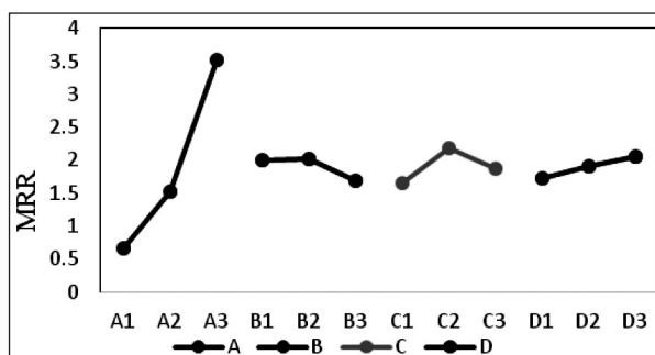
Fig. 2. Response graph for material removal rate.
